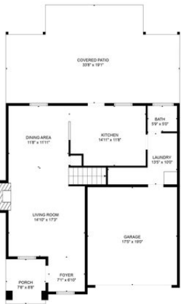
FLOOR PLAN CREATED BY CUBICASA APP. MEASUREMENTS DEEMED HIGHLY RELIABLE BUT NOT GUARANTEED. Copyright 2025 San Antonio Board of Realtors®
